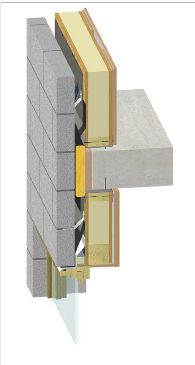
Figure 5 Infill panel
